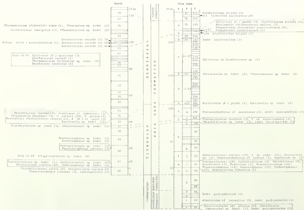
TEXT-FIG. 4. Vertical sections of the Chia Gara Formation in the type section on Chia Gara, and at Banik. In the Chia Gara section all the different systems of bed numbers that have been used are compared: the column labelled A shows the series of letters used by Wetzel (1959, pp. 72-74) when he designated this as type section; B shows the series of letters a-x used by Spath (1950, pp. 96-97) for the Kimmeridgian and Tithonian, followed by the numbers 1-38 used by him (Spath 1952, p. 31) for the Berriasian (bed x = bed 1 of these series); C gives Wetzel's original field numbers that are used in this paper. Note that the Banik section is about half as thick as the Chia Gara section, and that different vertical thickness scales are used.
